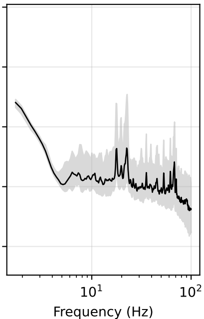
Logger 3376: noise PSD, 92 records
