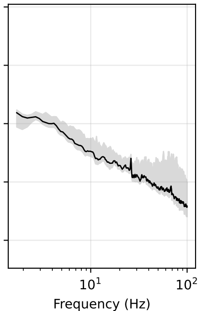
Logger 3274: noise PSD, 136 records
