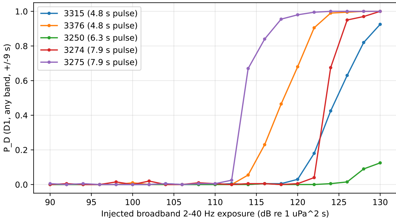
Injection-recovery into real IMOS background (200 per point)
