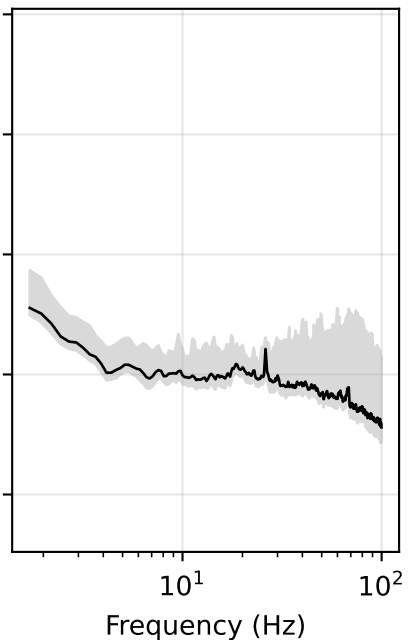
Logger 3275: noise PSD, 88 records
