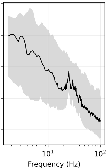
Logger 3250: noise PSD, 92 records
