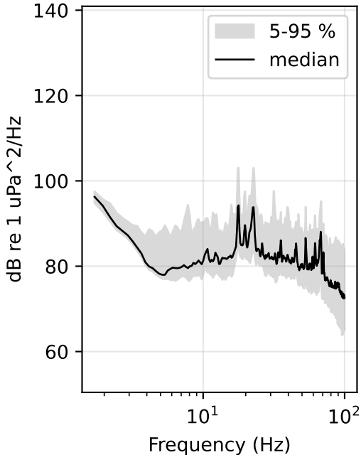
Logger 3315: noise PSD, 91 records
